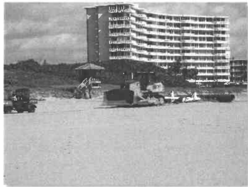
Beach fill operations at Delray Beach.
