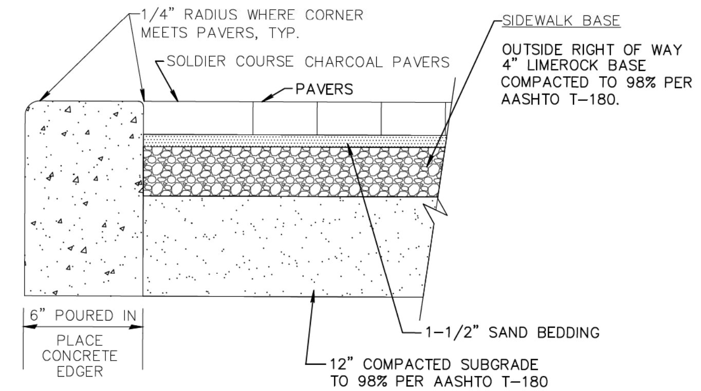
1 HS-1 CONC. PAVER WALKWAY-CITY STANDARD DETAIL N.T.S.
