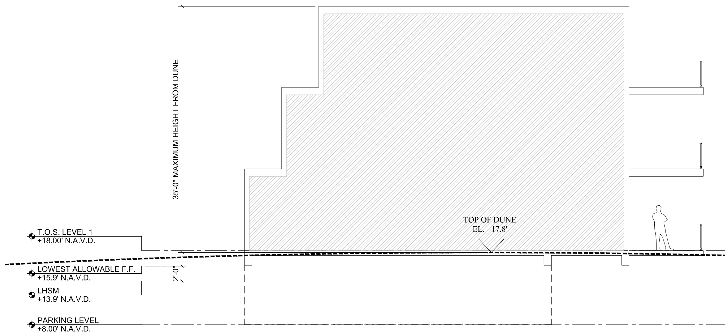
SECTION DIAGRAM
