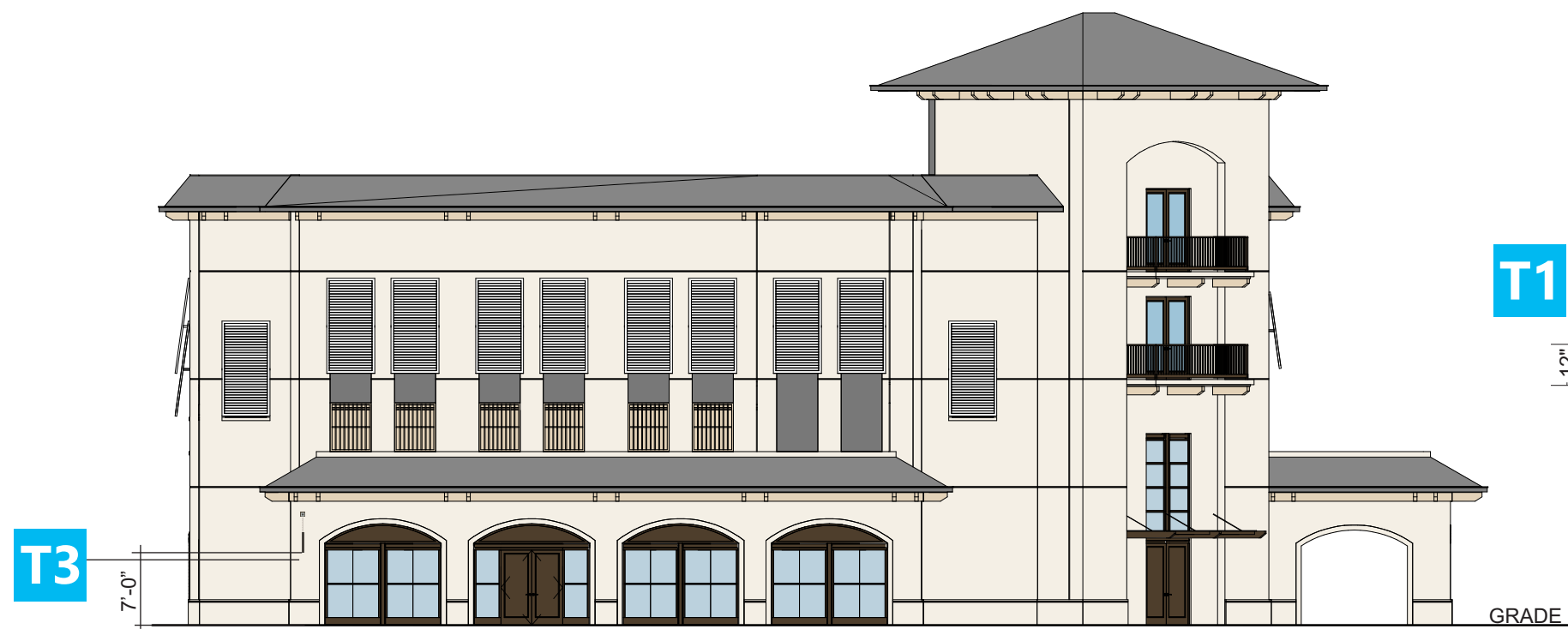
BLOCK 69 -PROPOSED EXTERIOR ELEVATION -SOUTH SCALE:1/16" = 1'-0"
