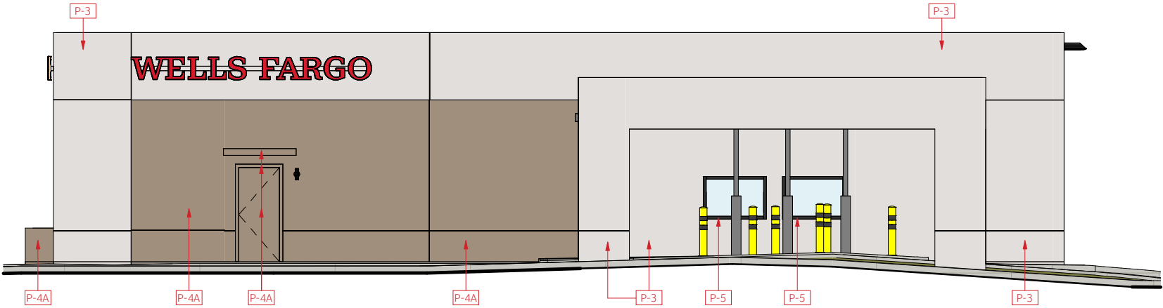
Proposed Color Exterior Elevation West View
