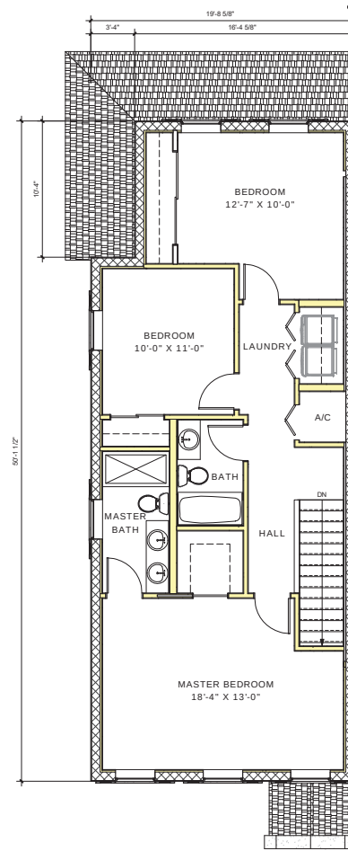
② 02-Second Floor Plan - TH-A 1/4" = 1'-0"
