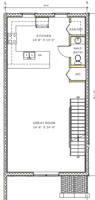
② 02-Second Floor Plan - TH-B1 1/4" = 1'-0"
