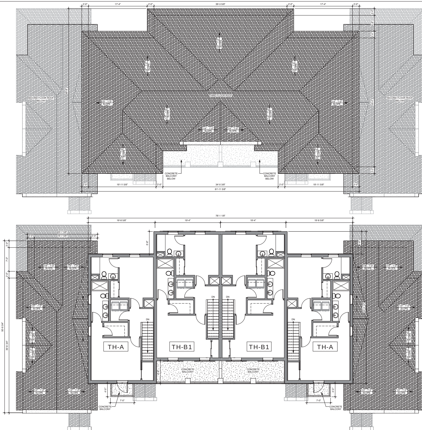
04-Roof Plan -Building Type 1 3/16" = 1'-0"
