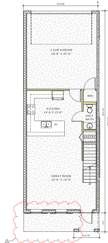
① 01-First Floor Plan - TH-A 1/4" = 1'-0"
