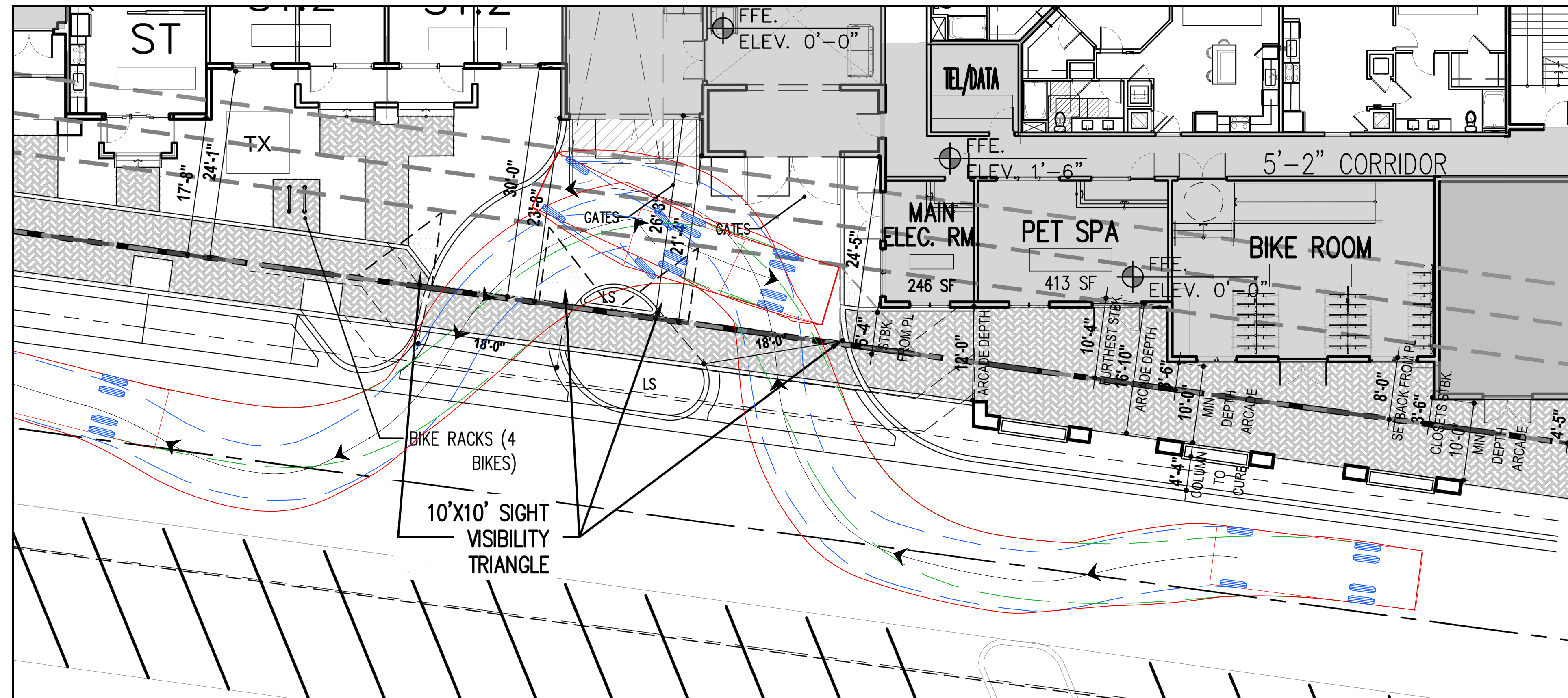
26' TRUCK SCALE 1"=10'
