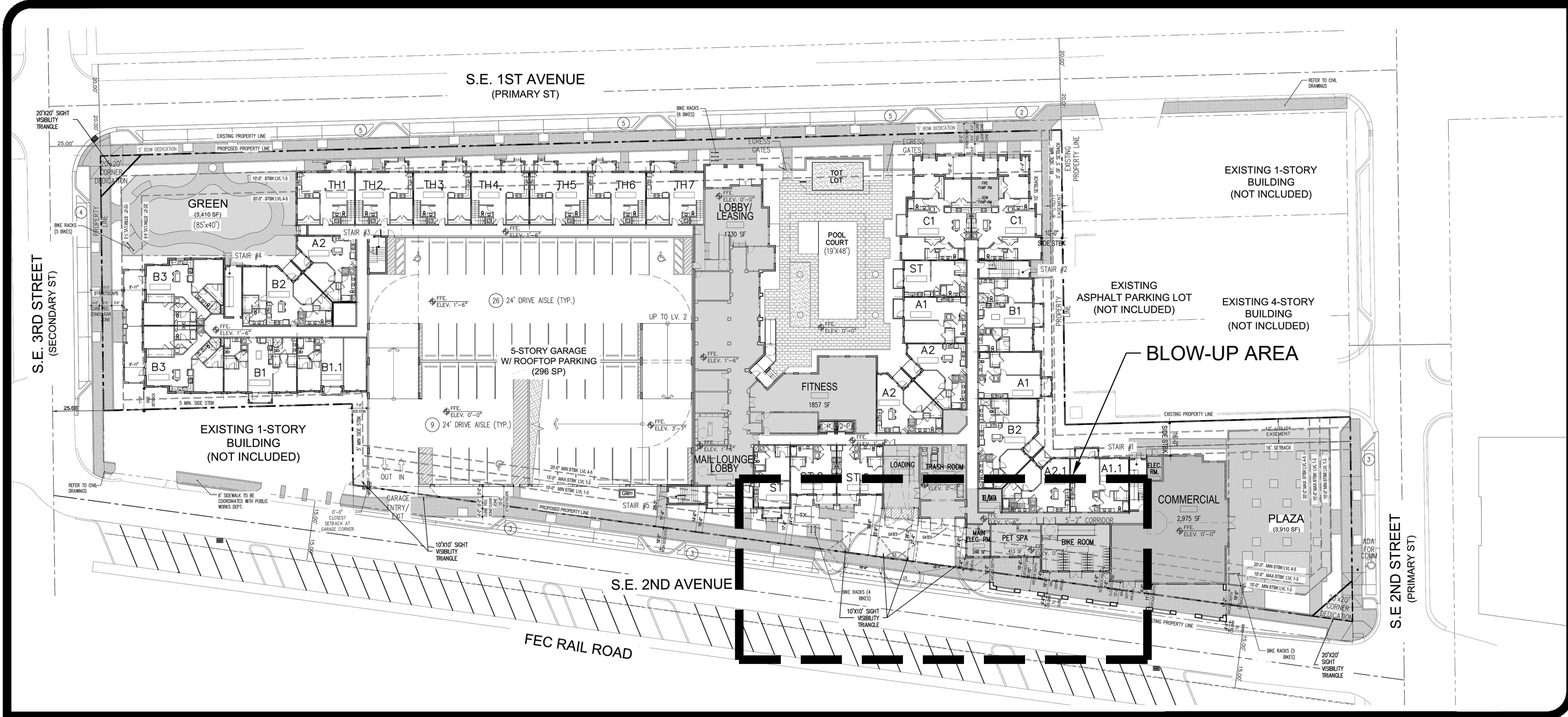
MASTER VIEW SCALE 1"=40'
