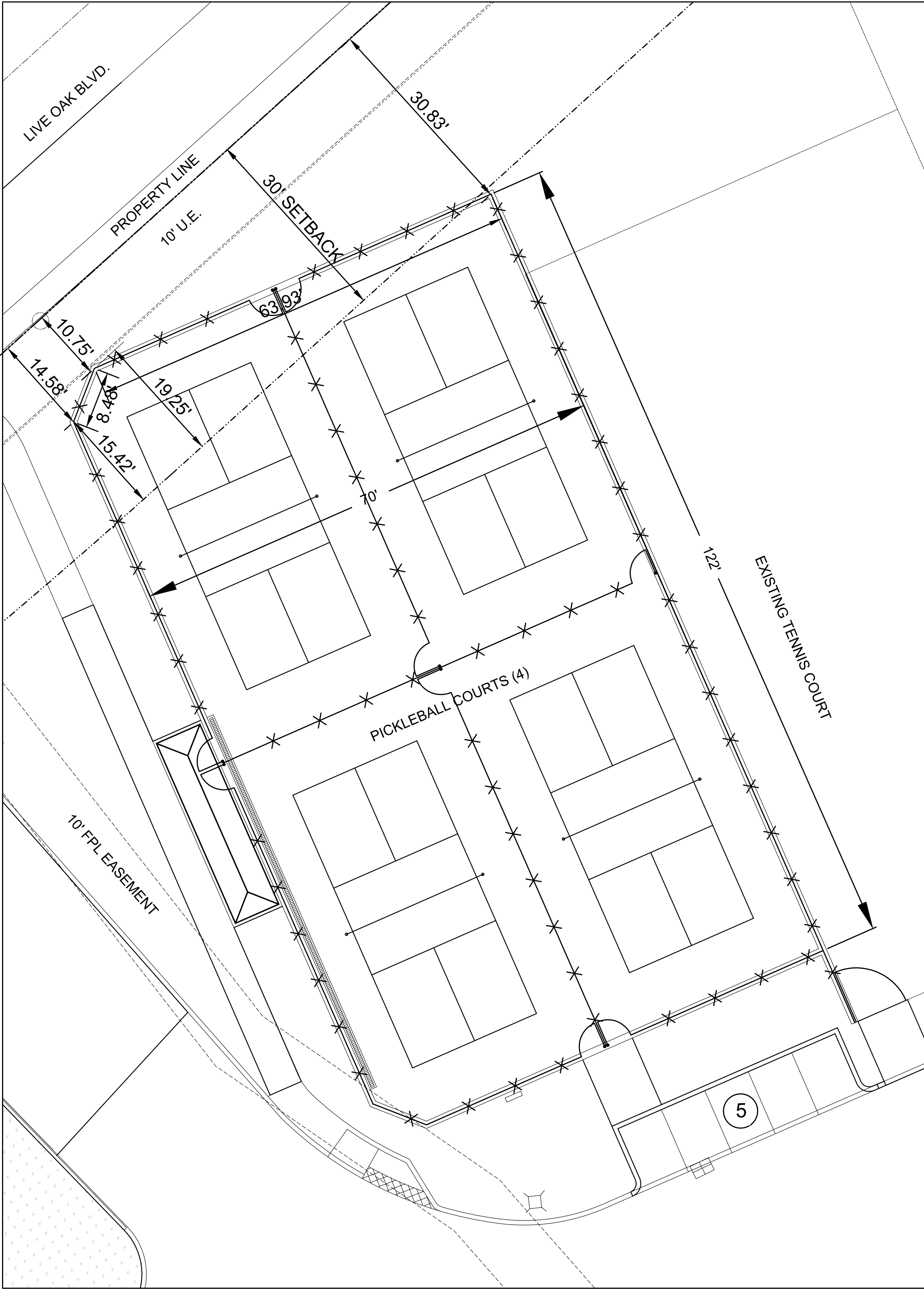
2023 APPROVED SITE PLAN
