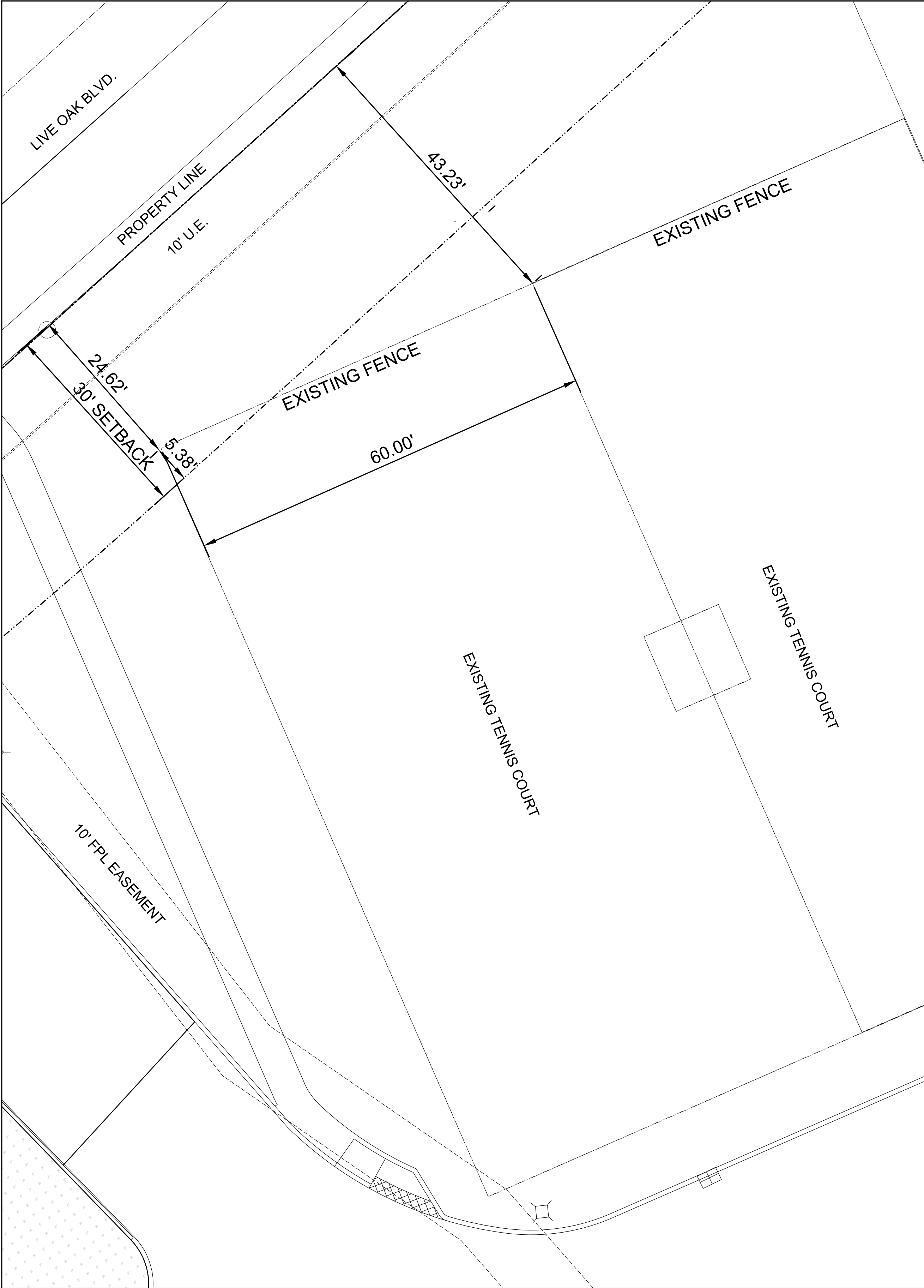
2022 APPROVED SITE PLAN
