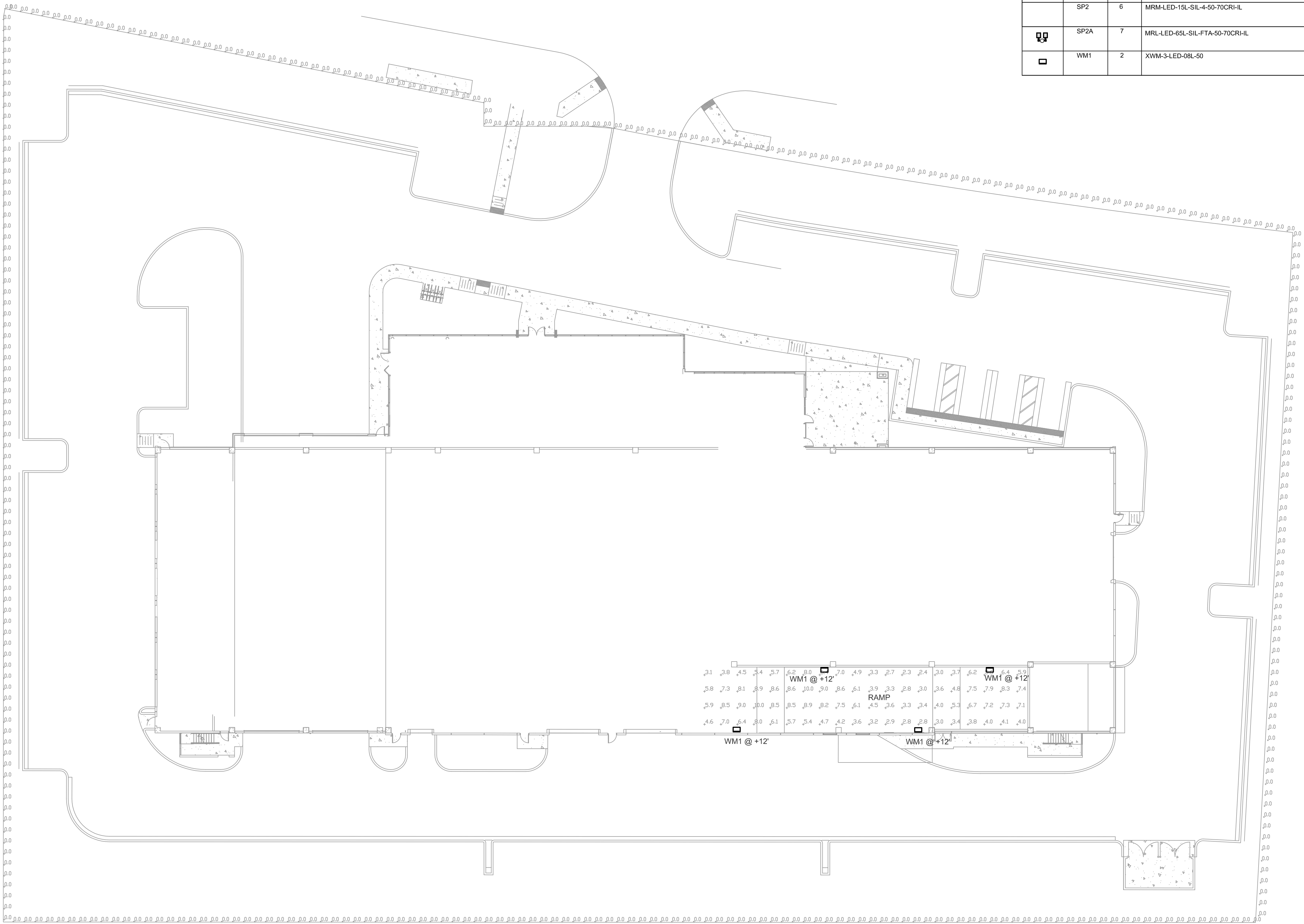
1 SITE PHOTOMETRIC PLAN - PARKING DECK - DAY SCALE: 1" = 20'-0"
