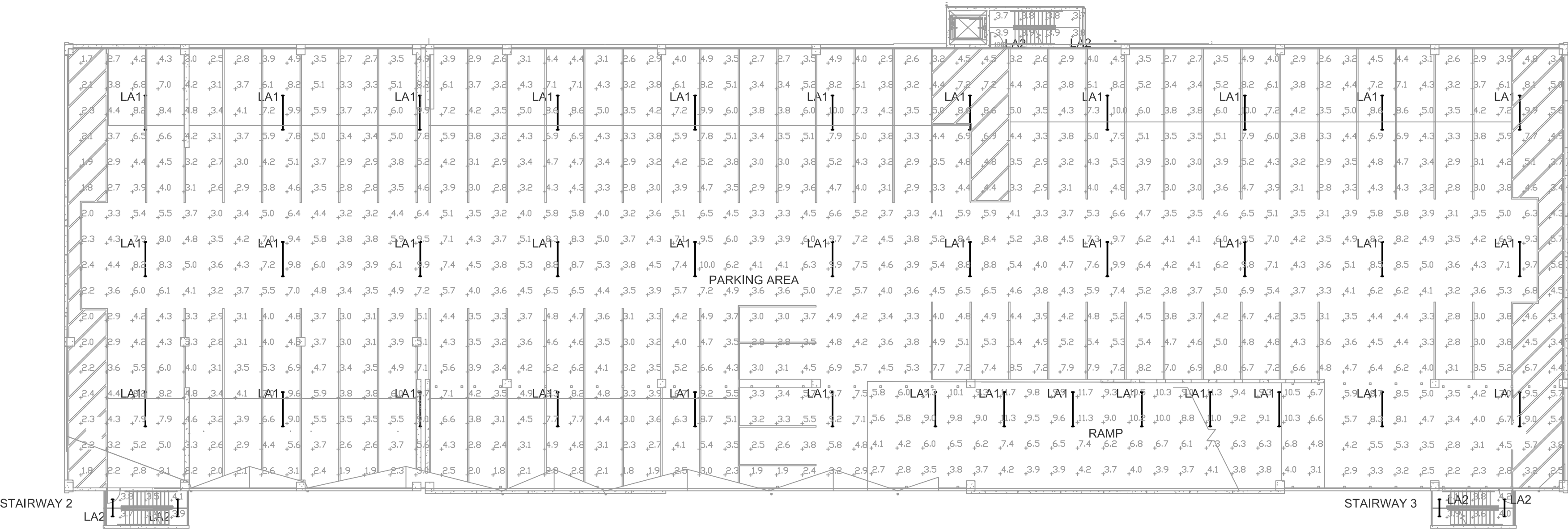
2 3rd LEVEL PARKING GARAGE PHOTOMETRIC PLAN - DAY SCALE: 1" = 20'-0"
