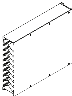
BACK PAN (INTERNAL VIEW)
