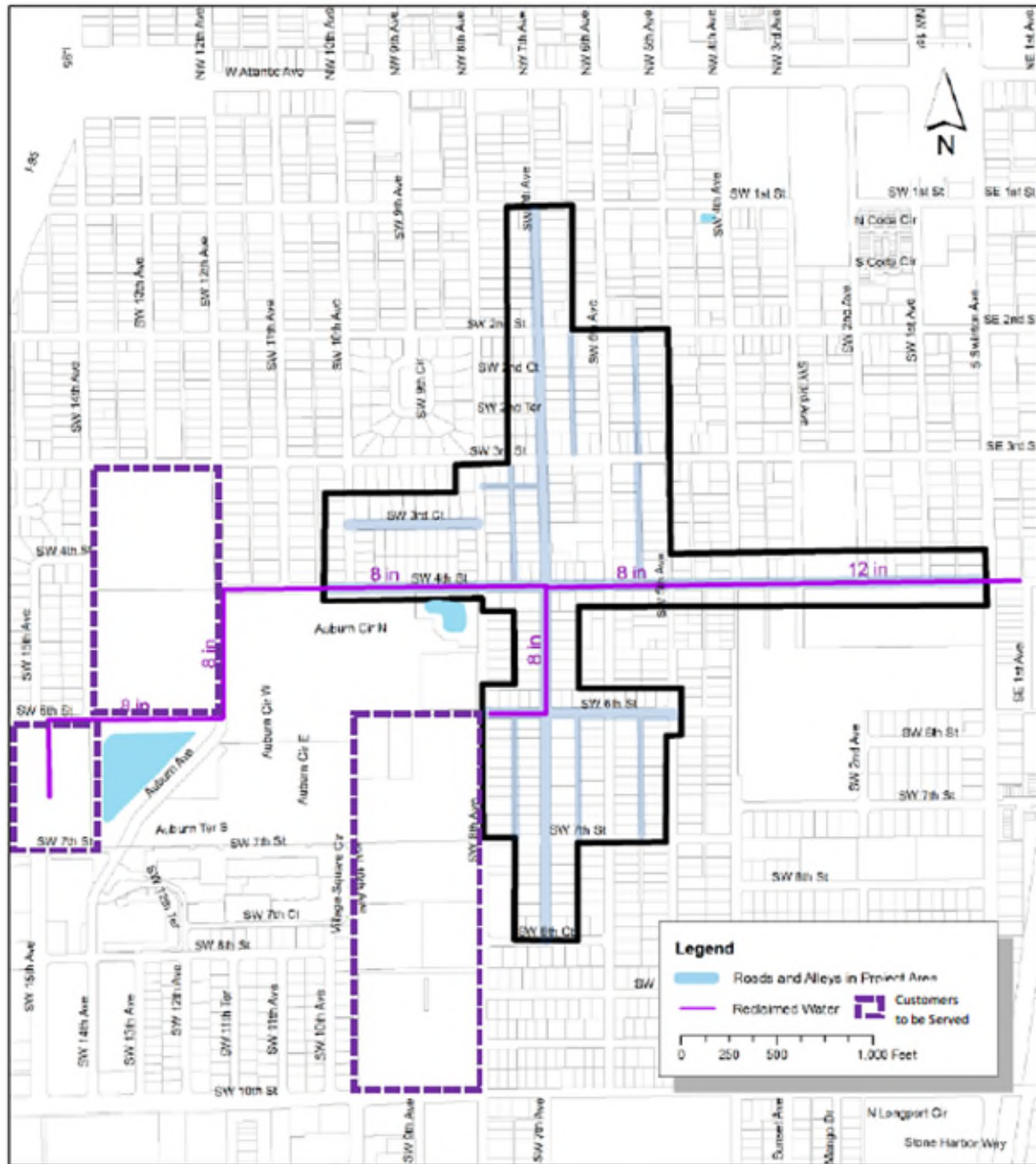
Figure 1. Proposed reclaimed water pipeline
