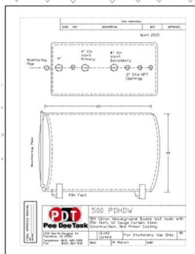
FUEL STORAGE CONTAINER
