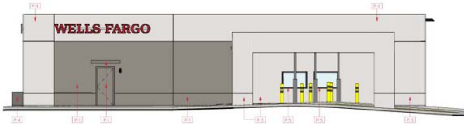
Proposed Color Exterior Elevation West View
