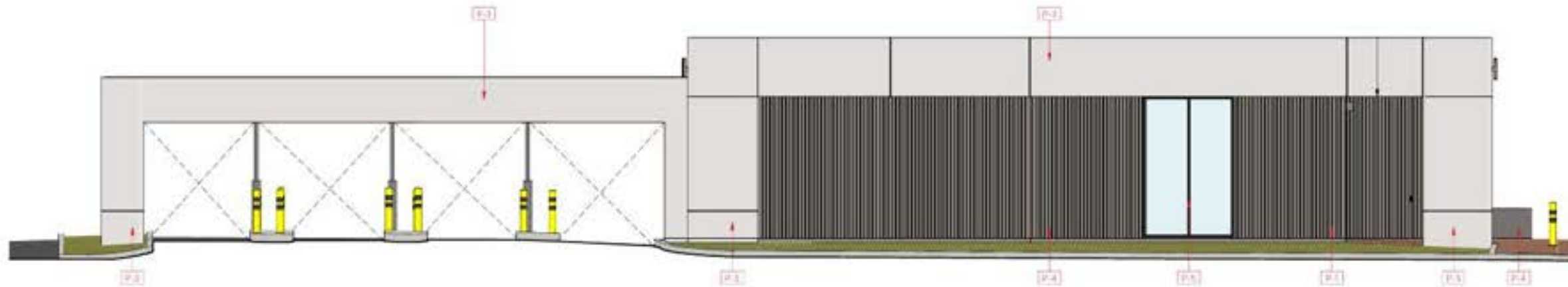
Proposed Color Exterior Elevation South View
