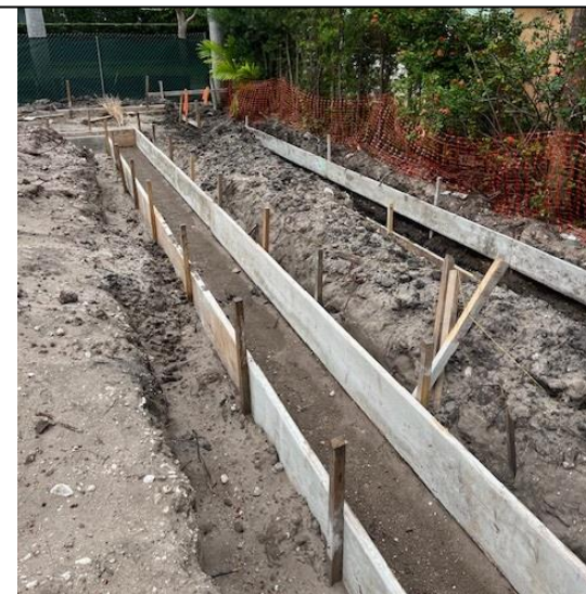
East wall footer formatted for east addition and retaining wall footers formatted for East Retaining wall to raise FEMA elevation
