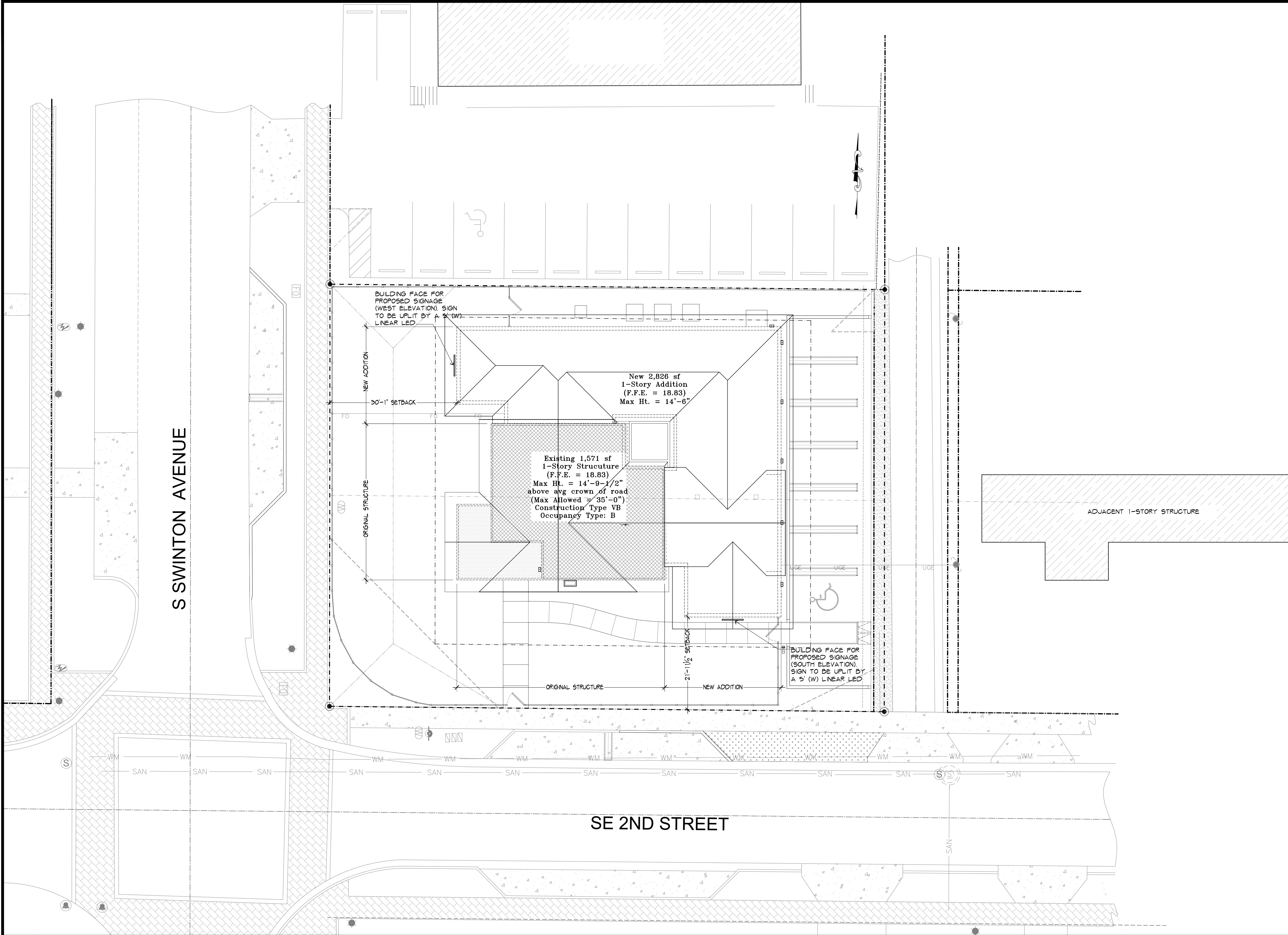
1 1" = 10'-0" SITE PLAN
