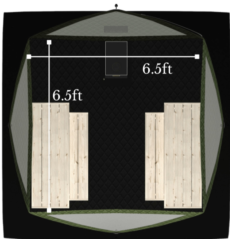
Top-down layout: stove position and bench placement (6.5 ft x 6.5 ft interior)
