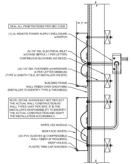
WALL MOUNTING DETAIL
