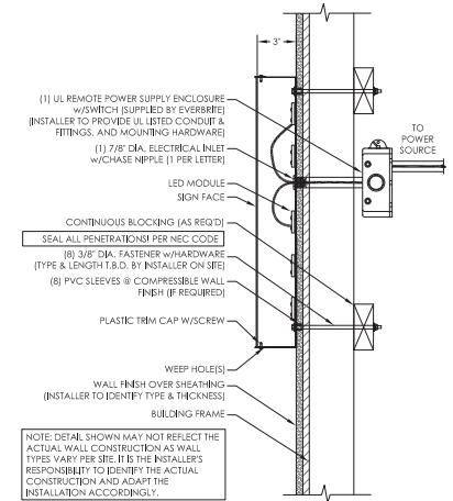
WALL MOUNTING DETAIL
