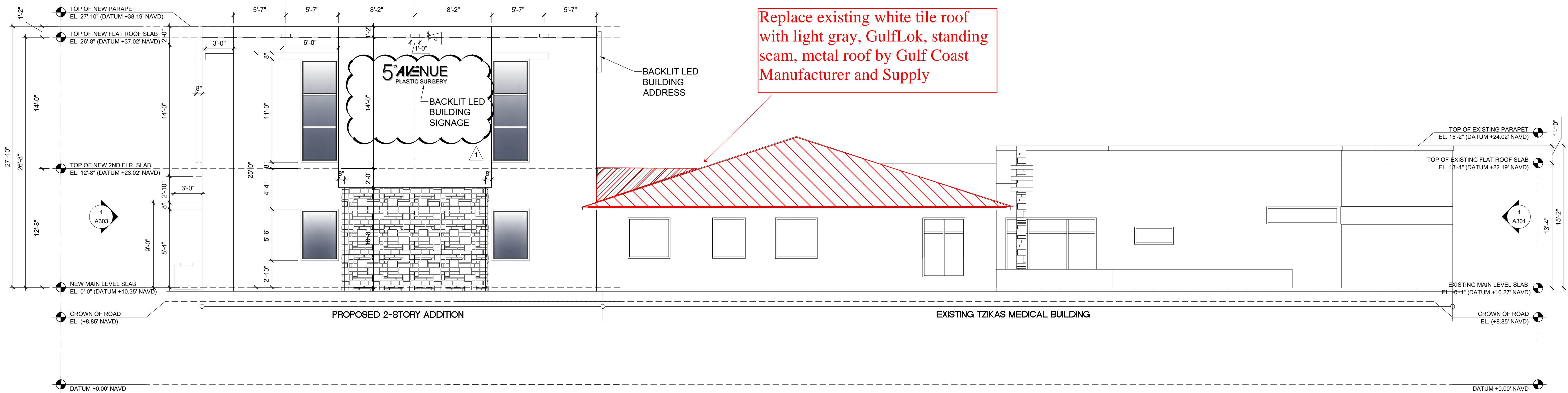
1 EAST ELEVATION 3/16"=1'-0"
