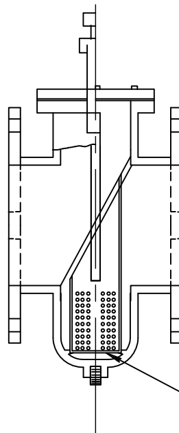
BASKET STRAINER
