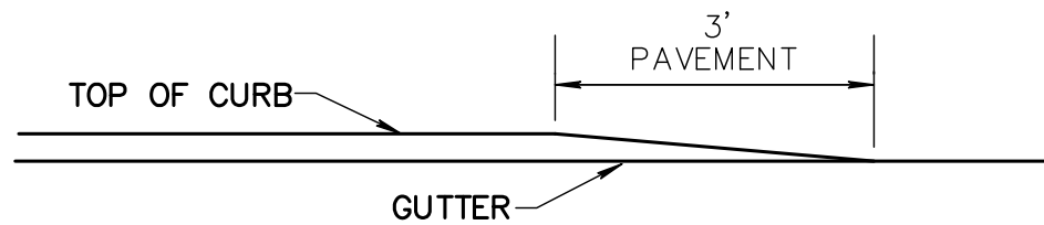
PROFILE
