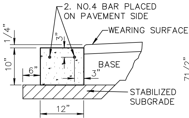
CONCRETE HEADER CURB NOT TO SCALE
