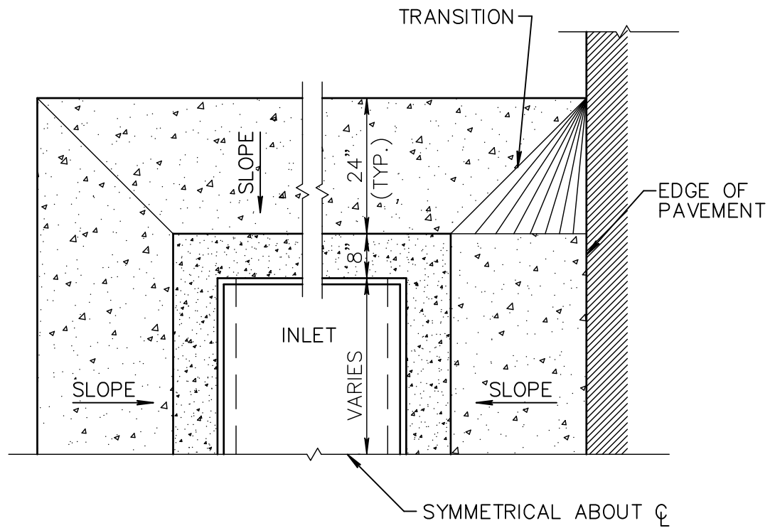
HALF PLAN
