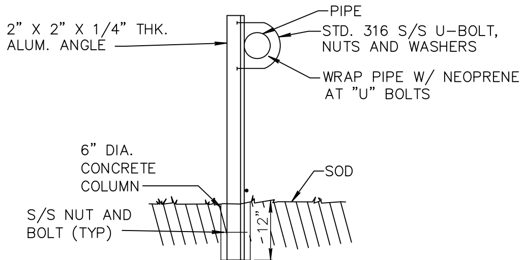
PIPE SUPPORT DETAIL
