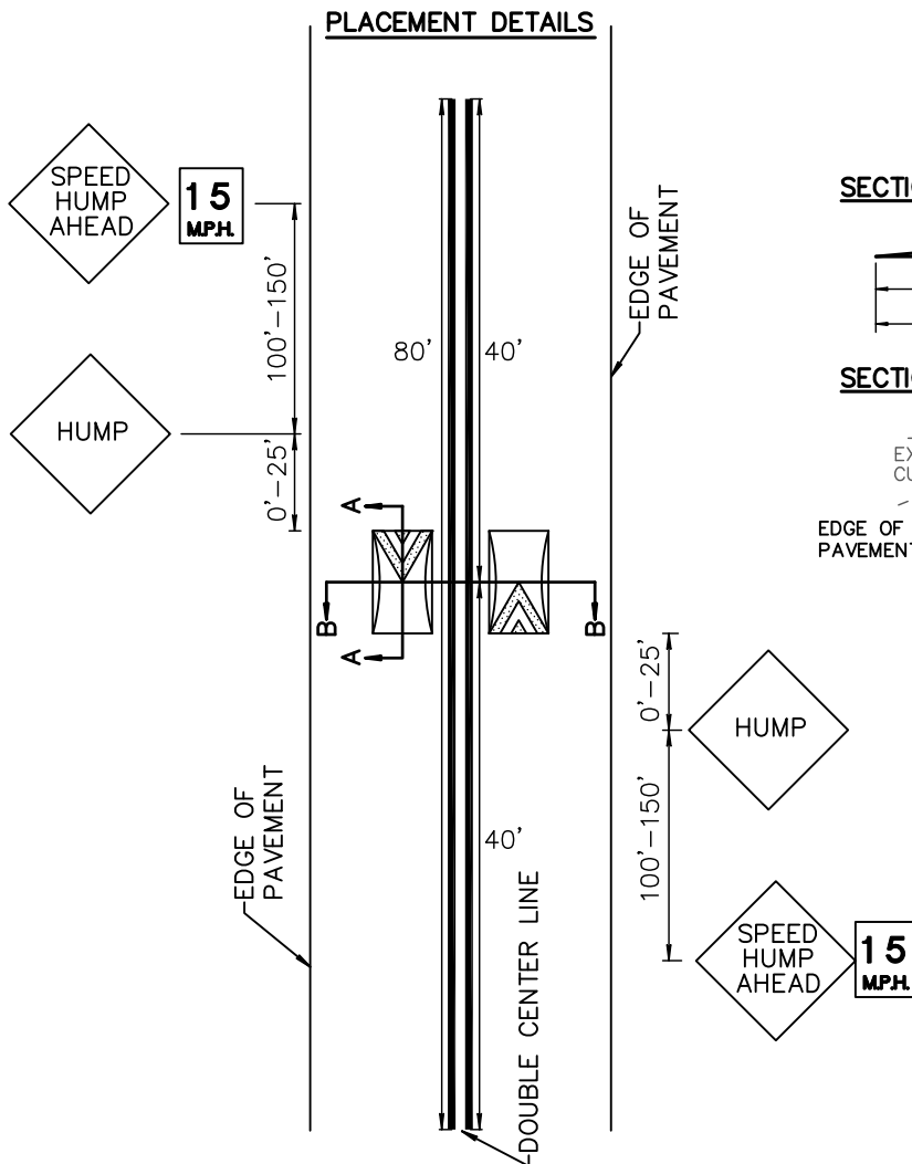
SIGNS AND MARKINGS DETAILS
