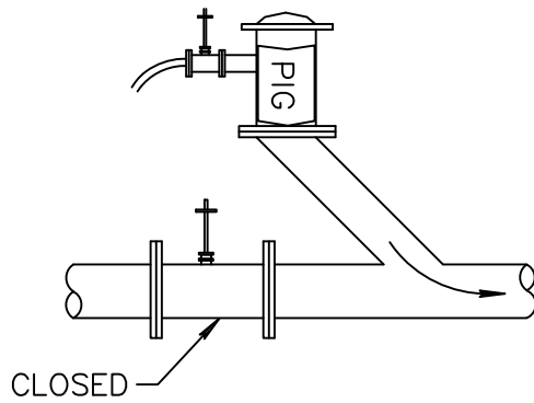
WYE ENTRY
