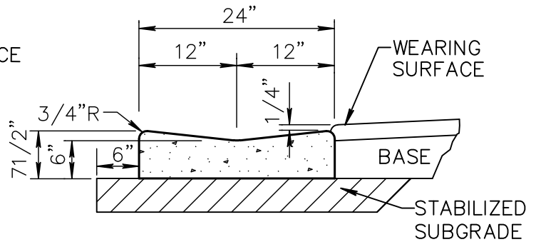
VALLEY GUTTER NOT TO SCALE
