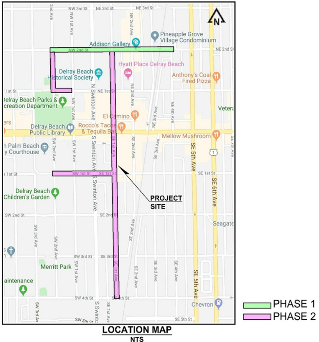
Figure 1. Proposed Phase 2 reclaimed water pipeline
