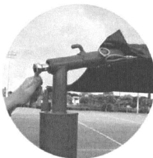
Step 2: Turn concealed nut using a standard socket wrench. Attachment hook moves backward, releasing the canopy cables.
