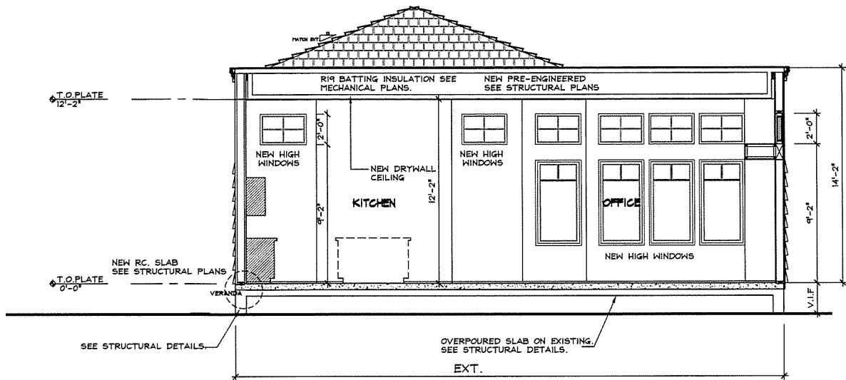
SECTION C-C
