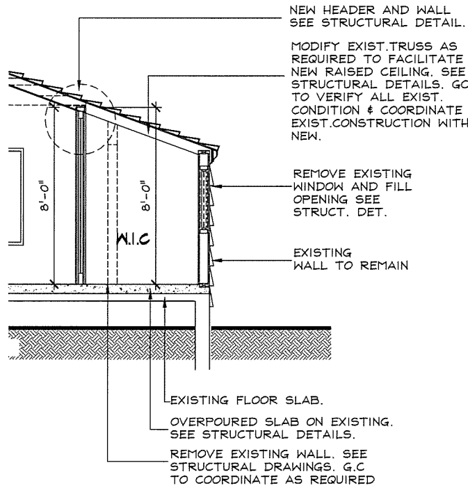
SECTION 'D'
