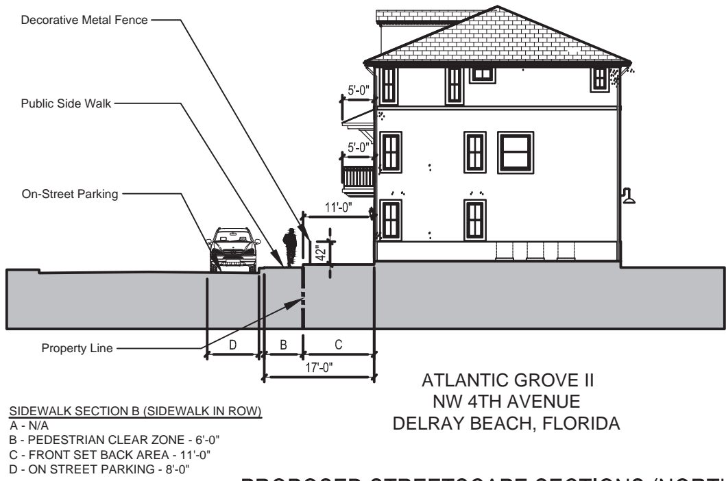
PROPOSED STREETSCAPE SECTIONS (NORTH) SCALE: N.T.S.
