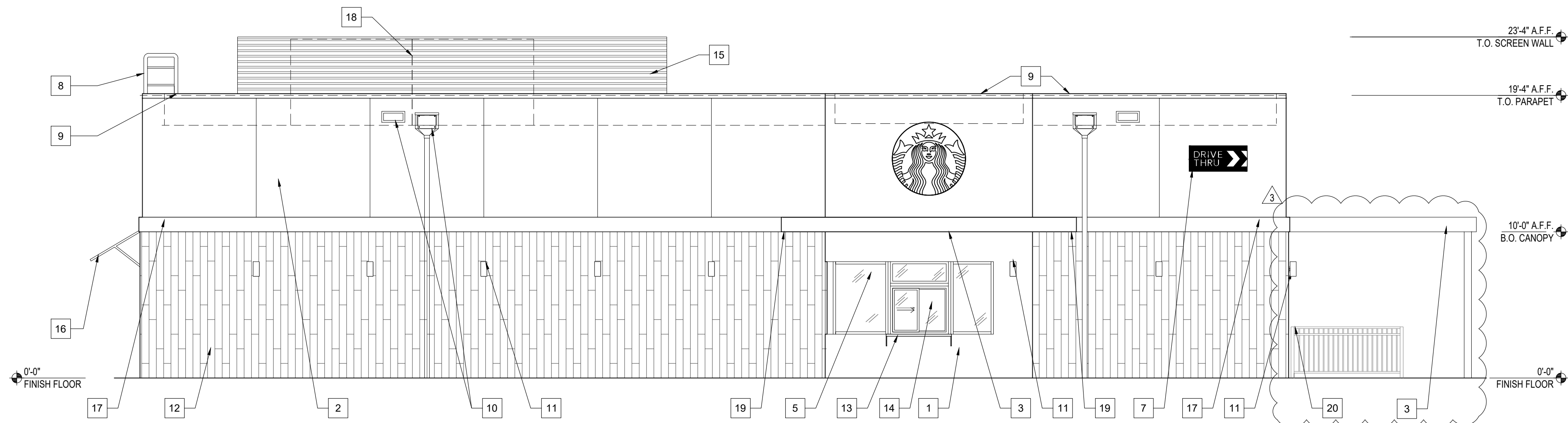
04 SOUTH ELEVATION SCALE: 3/16" = 1'-0"
