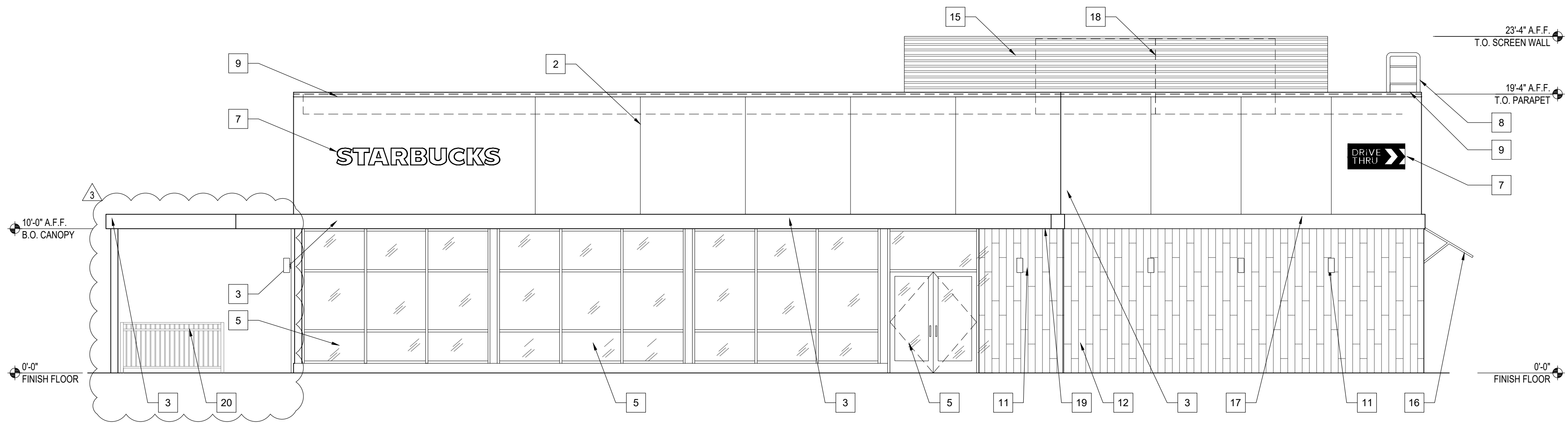
01 NORTH ELEVATION SCALE: 3/16" = 1'-0"
