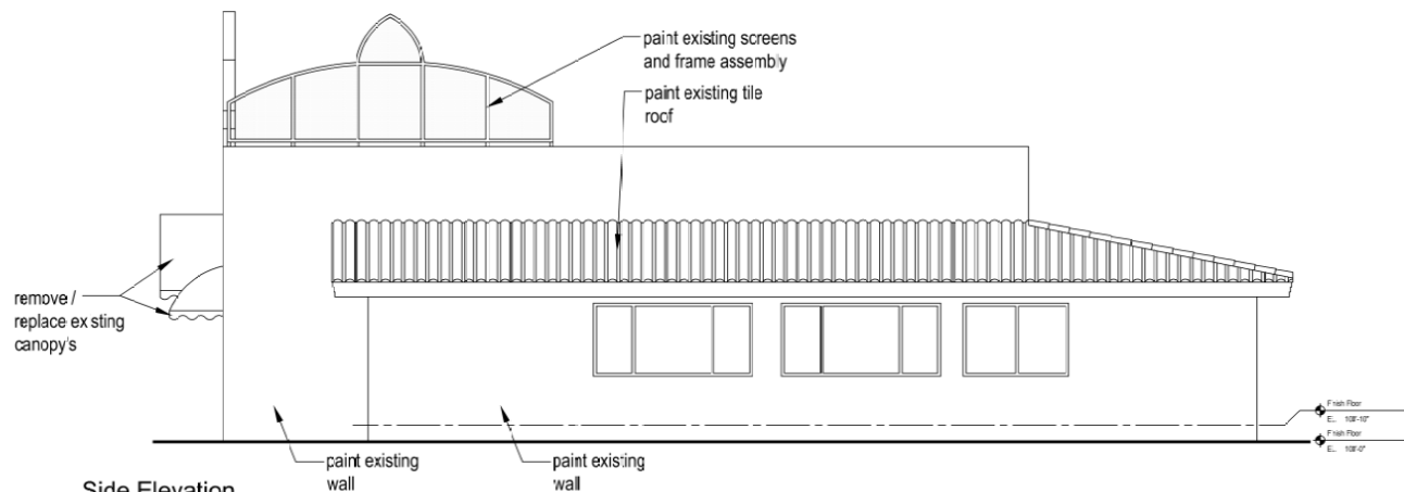
Side Elevation Looking North Scale: NTS
