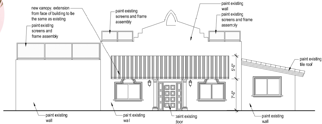
Front Elevation 2nd Avenue View Scale: 1/8" = 1'-0"
