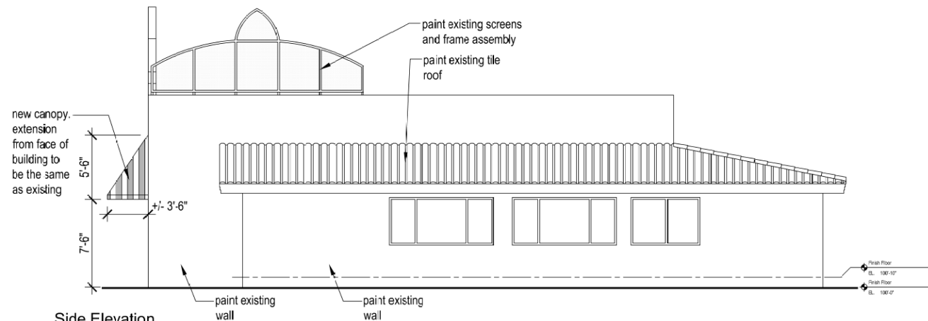
Side Elevation Looking North Scale: 1/8" = 1'-0"
