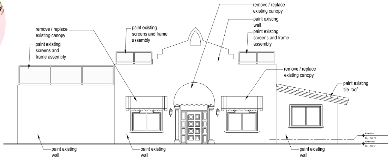
Front Elevation 2nd Avenue View Scale: NTS
